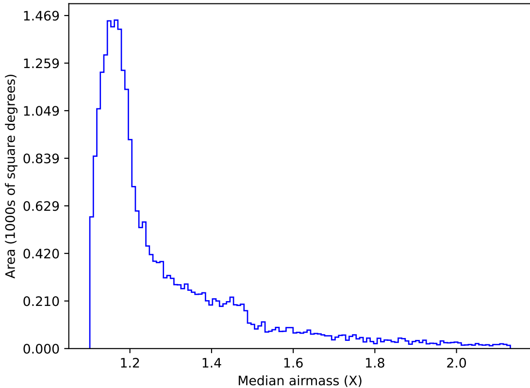
all_long_v3.4_10yrs All sky i band: Median airmass
