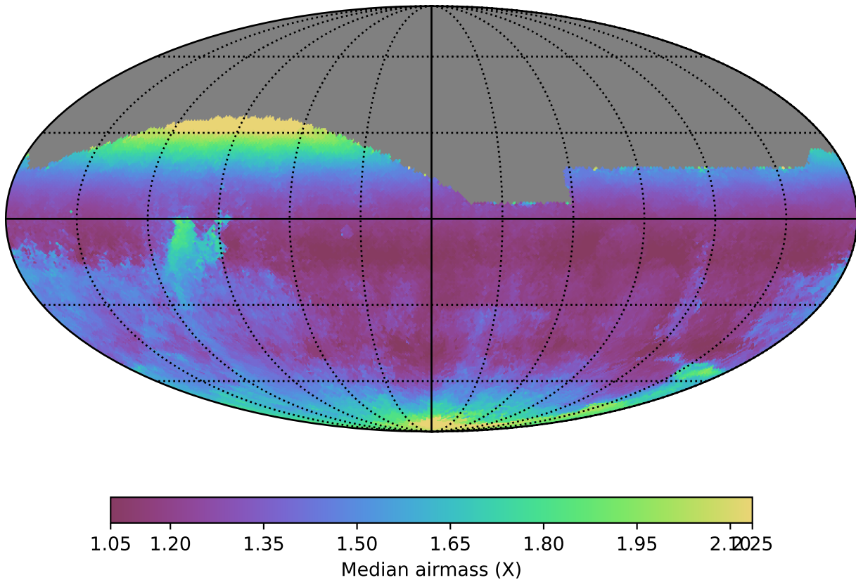
all_long_v3.4_10yrs All sky g band: Median airmass
