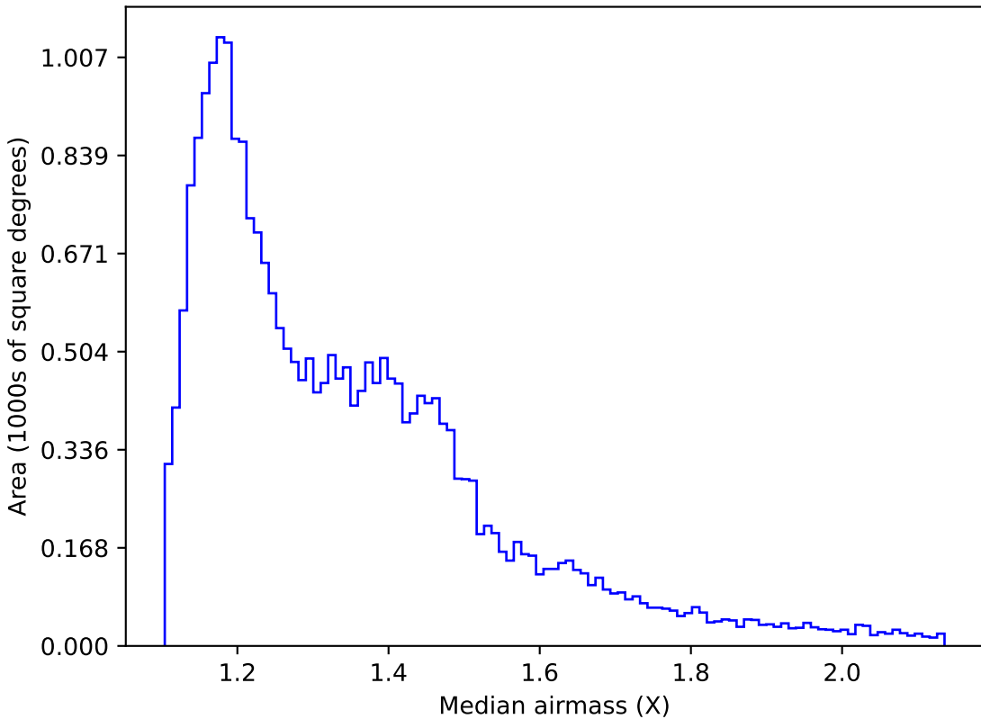
all_long_v3.4_10yrs All sky g band: Median airmass
