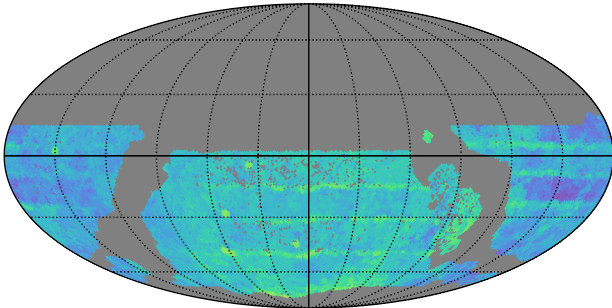
all_long_v3.4_10yrs WFD z band: Median Season Length
