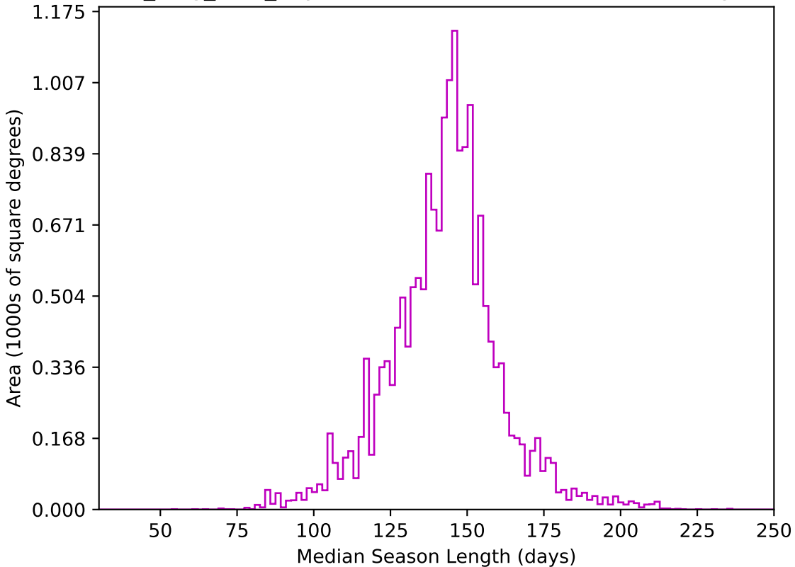
all_long_v3.4_10yrs WFD z band: Median Season Length
