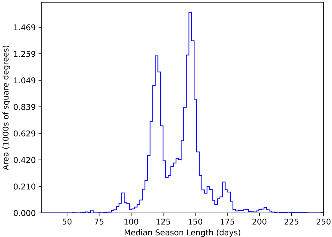
all_long_v3.4_10yrs WFD y band: Median Season Length
