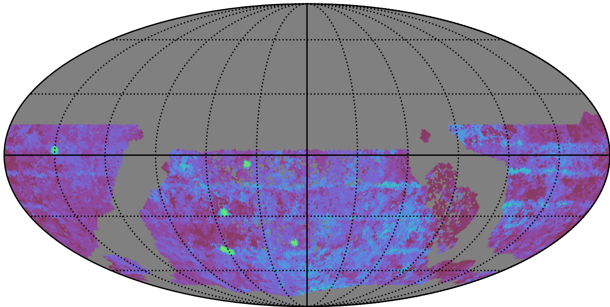
all_long_v3.4_10yrs WFD u band: Median Season Length
