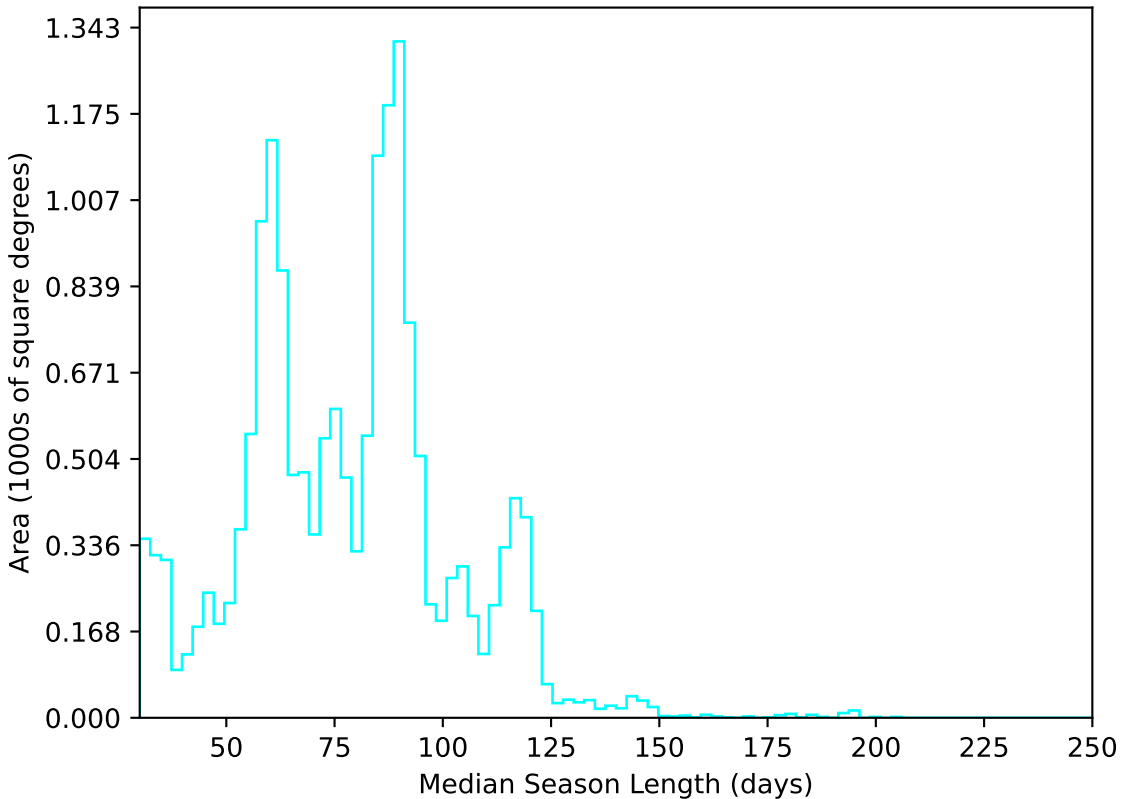
all_long_v3.4_10yrs WFD u band: Median Season Length
