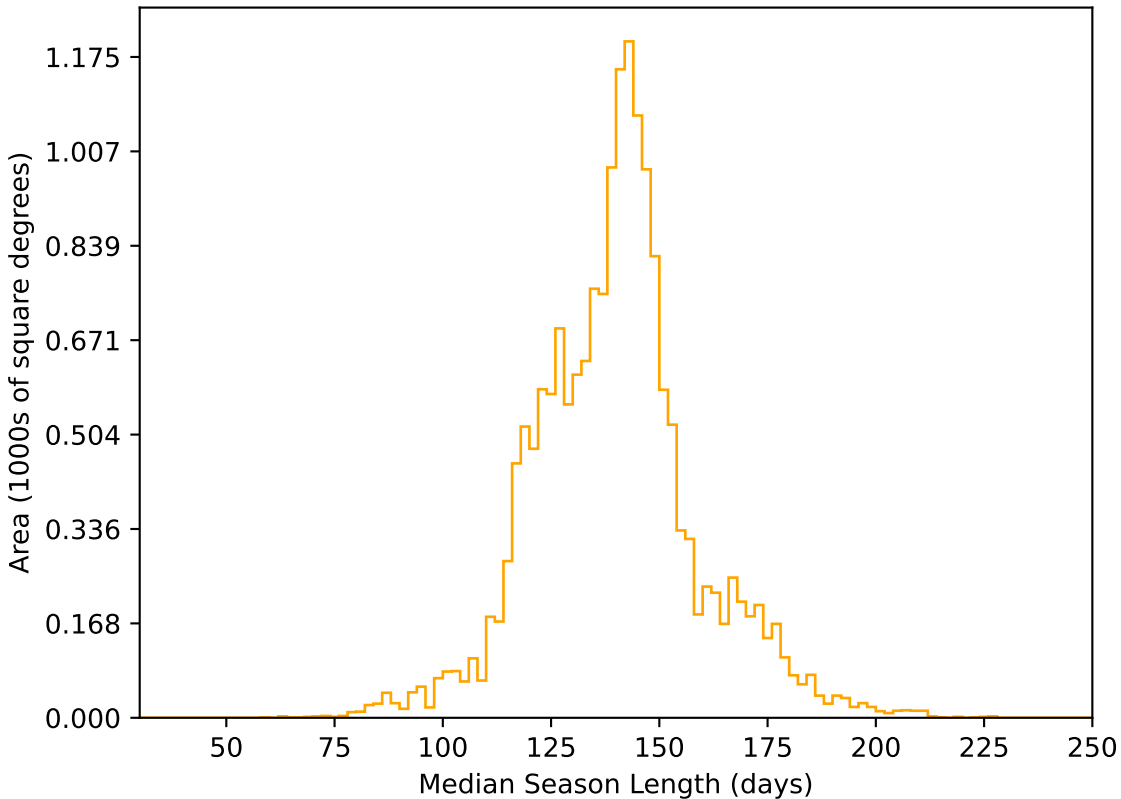
all_long_v3.4_10yrs WFD r band: Median Season Length
