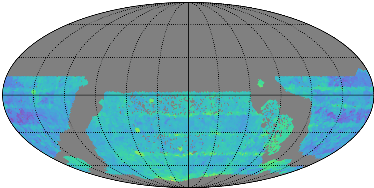
all_long_v3.4_10yrs WFD i band: Median Season Length
