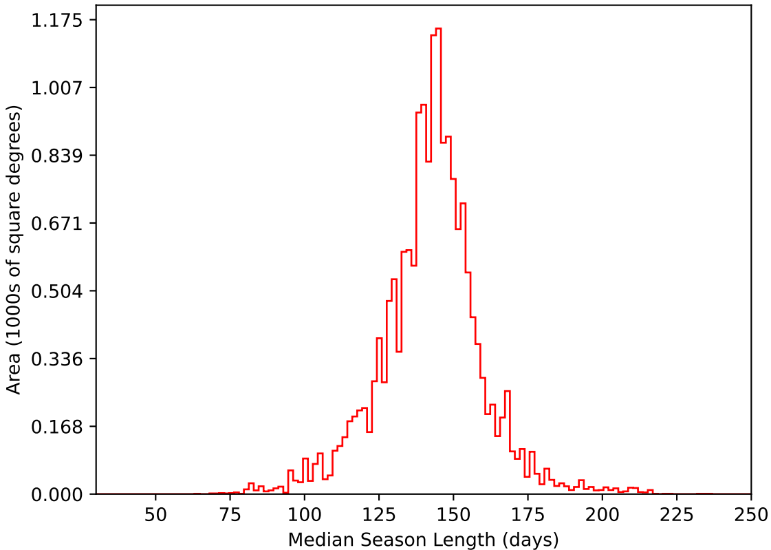
all_long_v3.4_10yrs WFD i band: Median Season Length
