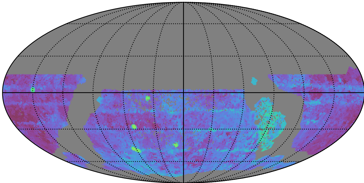
all_long_v3.4_10yrs WFD g band: Median Season Length
