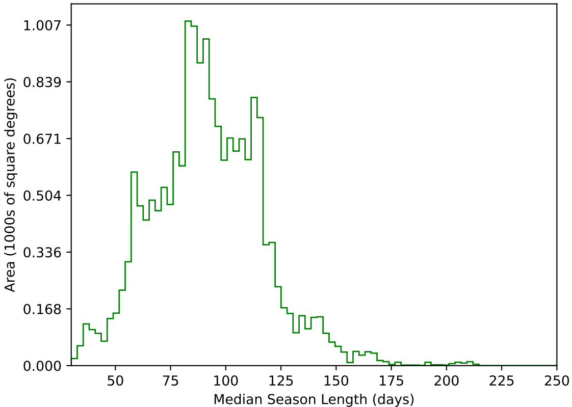
all_long_v3.4_10yrs WFD g band: Median Season Length
