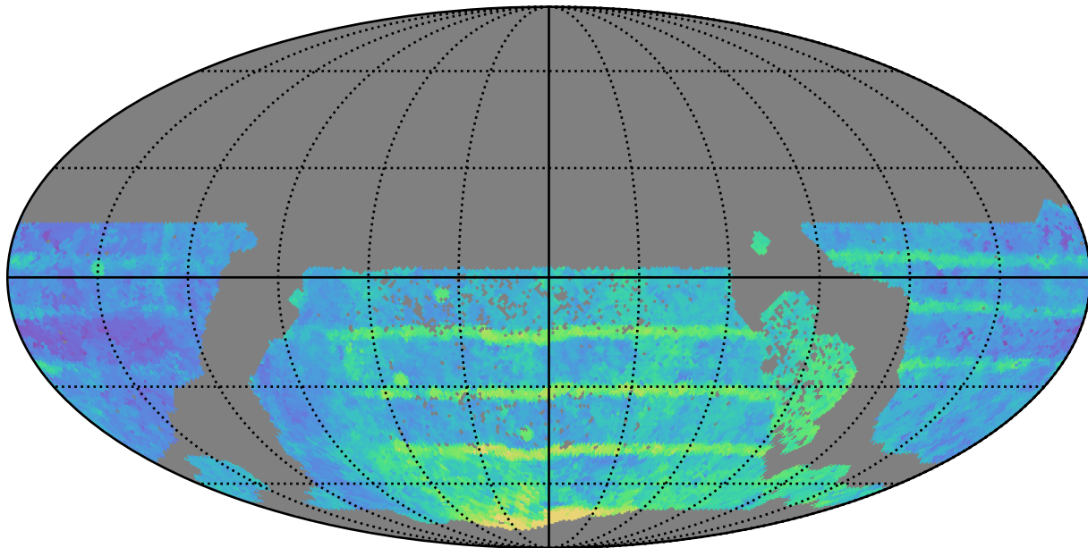
all_long_v3.4_10yrs WFD all bands: Median Season Length
