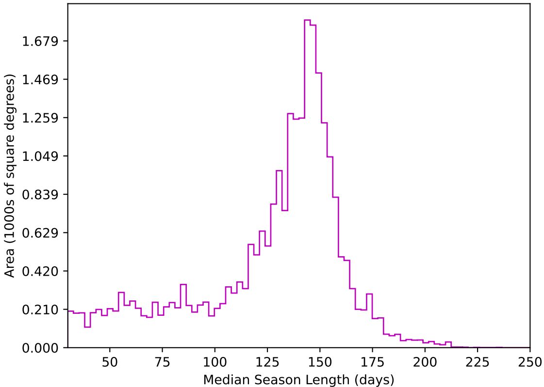
all_long_v3.4_10yrs All sky z band: Median Season Length
