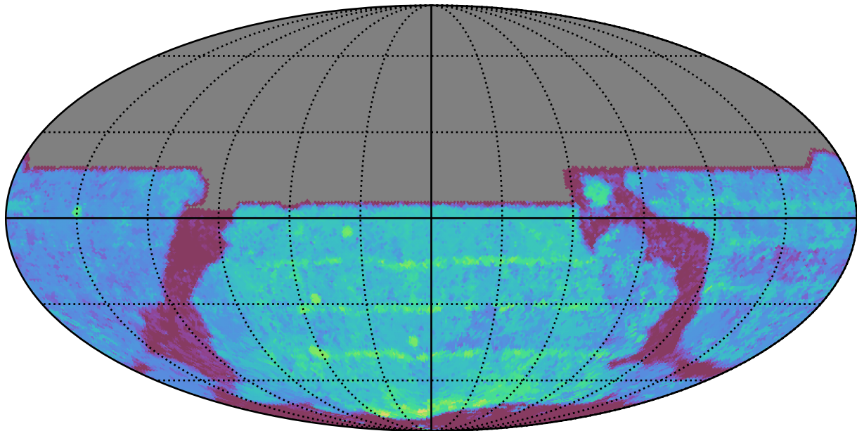
all_long_v3.4_10yrs All sky y band: Median Season Length
