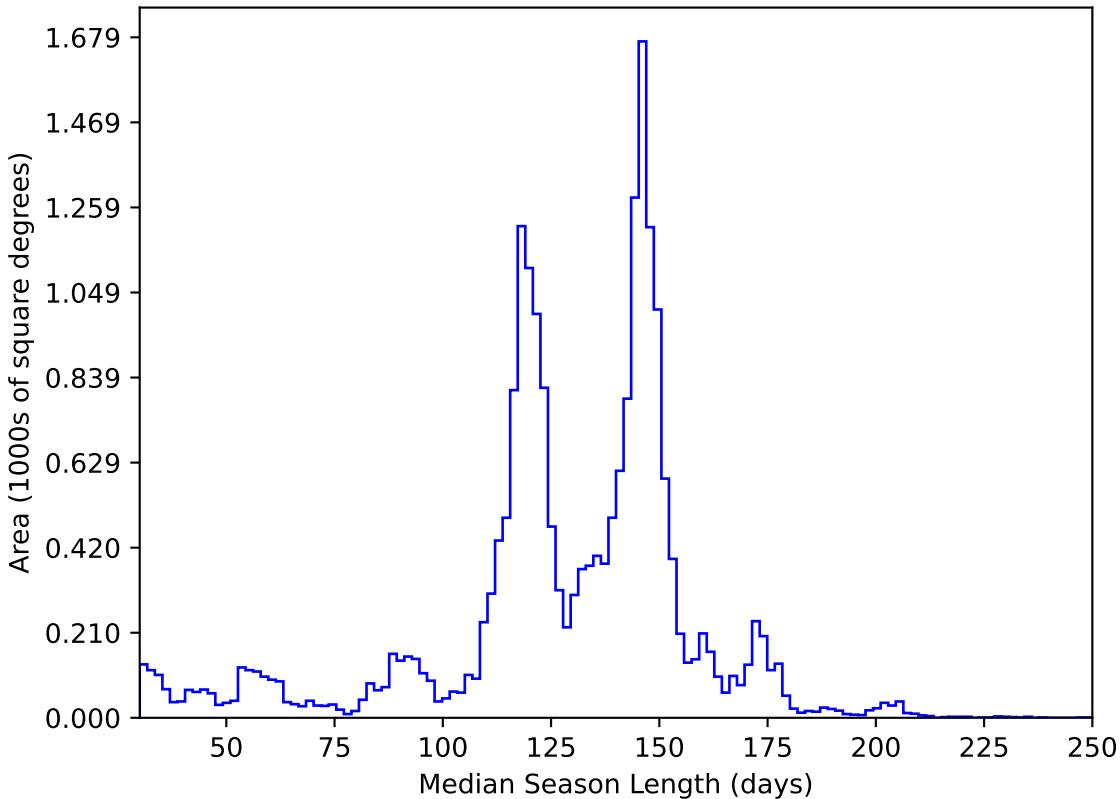
all_long_v3.4_10yrs All sky y band: Median Season Length
