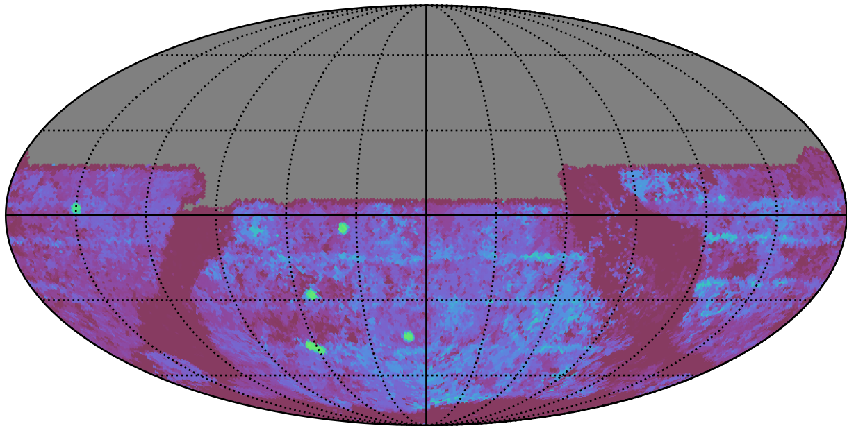
all_long_v3.4_10yrs All sky u band: Median Season Length
