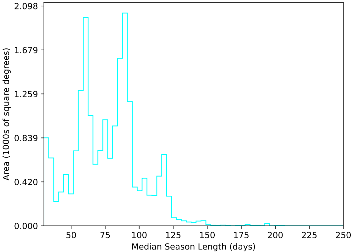
all_long_v3.4_10yrs All sky u band: Median Season Length
