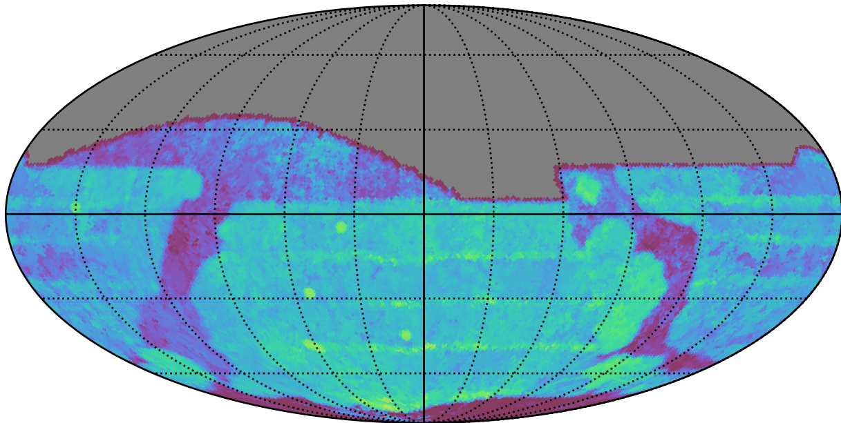
all_long_v3.4_10yrs All sky i band: Median Season Length
