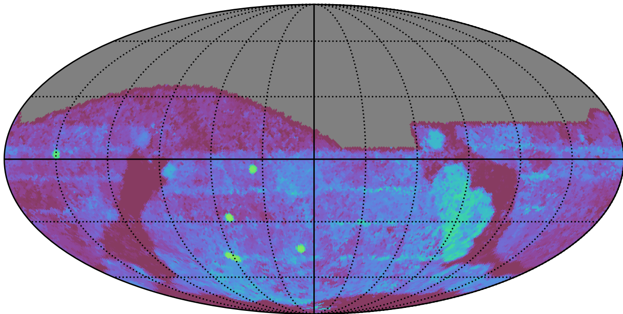
all_long_v3.4_10yrs All sky g band: Median Season Length
