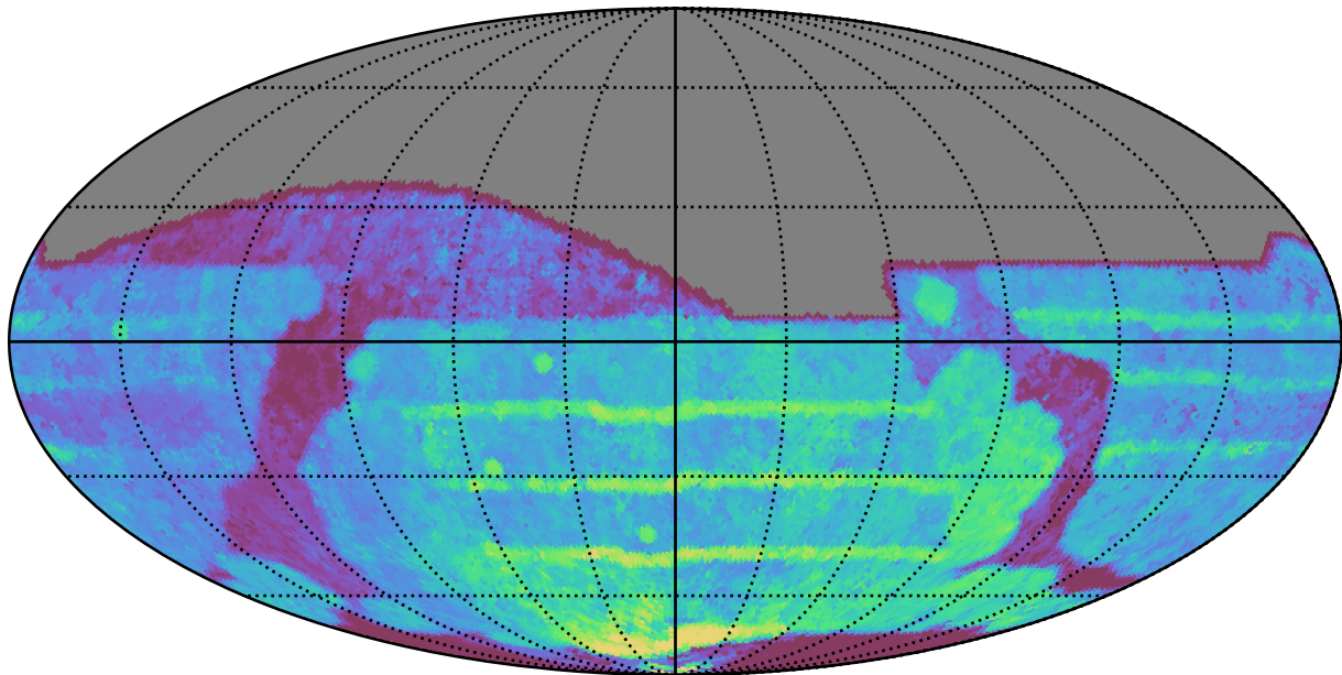
all_long_v3.4_10yrs All sky all bands: Median Season Length
