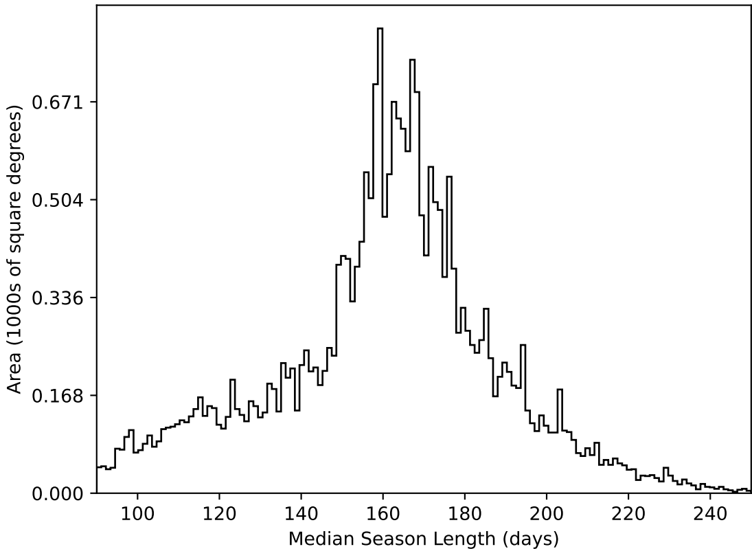
all_long_v3.4_10yrs All sky all bands: Median Season Length
