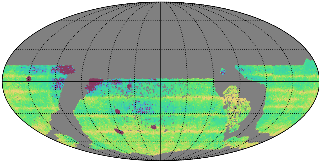
all_long_v3.4_10yrs WFD: Median Intra-Night Gap
