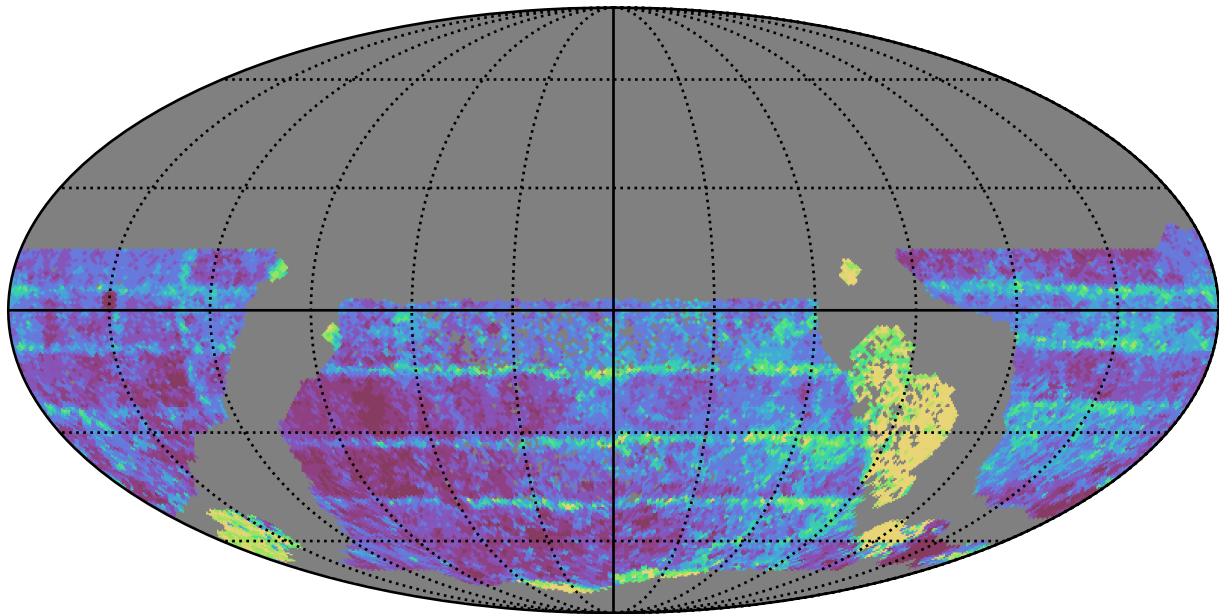
all_long_v3.4_10yrs WFD z band: Median Inter-Night Gap
