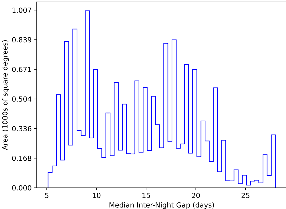
all_long_v3.4_10yrs WFD y band: Median Inter-Night Gap
