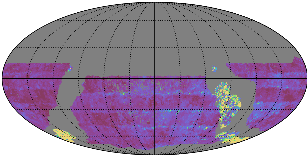
all_long_v3.4_10yrs WFD u band: Median Inter-Night Gap
