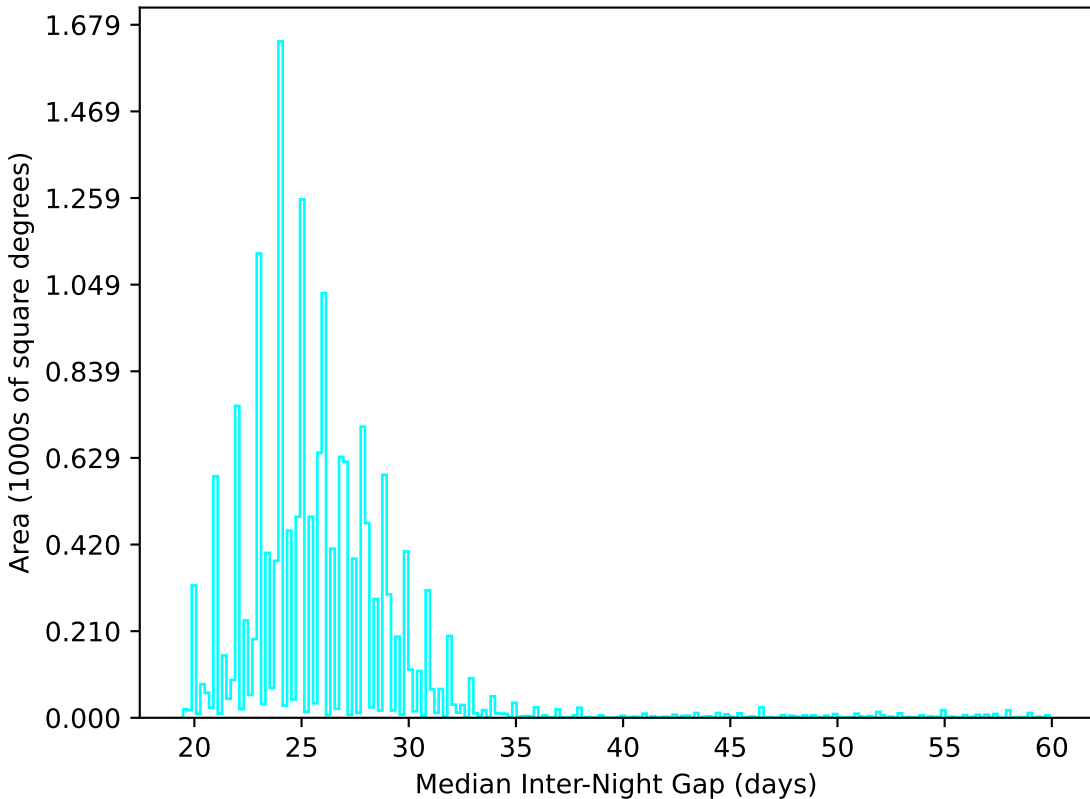
all_long_v3.4_10yrs WFD u band: Median Inter-Night Gap
