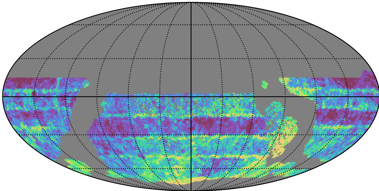
all_long_v3.4_10yrs WFD r band: Median Inter-Night Gap
