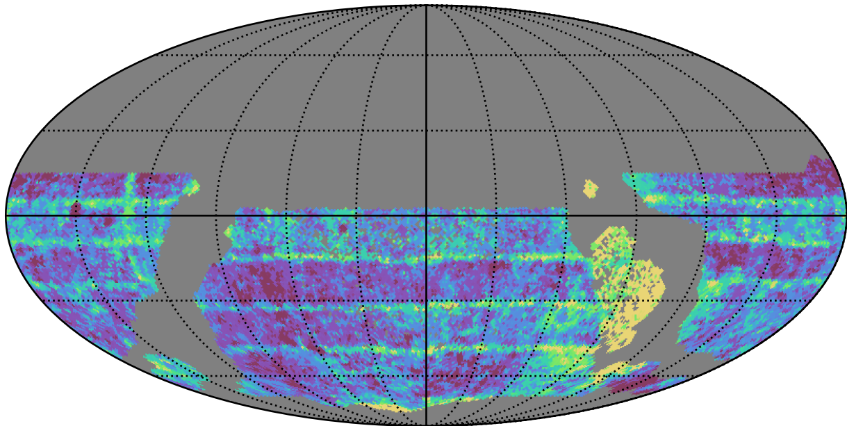
all_long_v3.4_10yrs WFD i band: Median Inter-Night Gap
