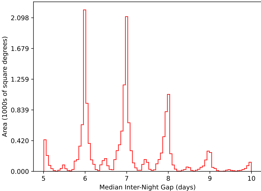
all_long_v3.4_10yrs WFD i band: Median Inter-Night Gap
