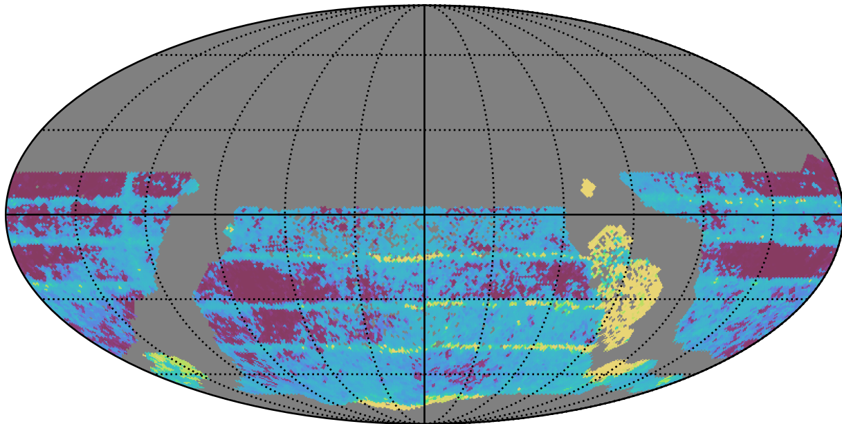
all_long_v3.4_10yrs WFD all bands: Median Inter-Night Gap
