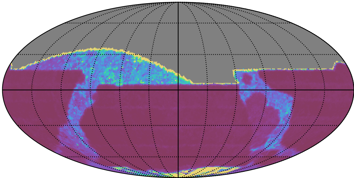
all_long_v3.4_10yrs All sky z band: Median Inter-Night Gap
