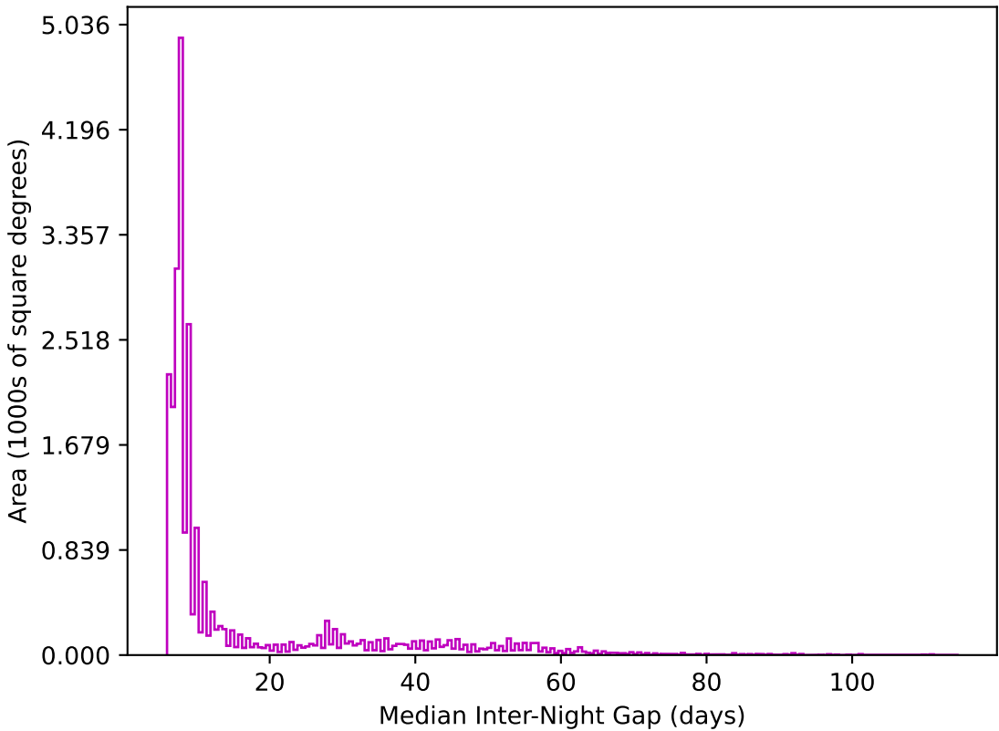
all_long_v3.4_10yrs All sky z band: Median Inter-Night Gap
