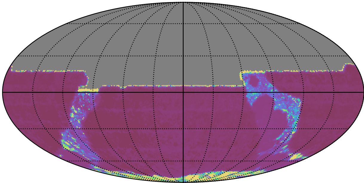
all_long_v3.4_10yrs All sky y band: Median Inter-Night Gap
