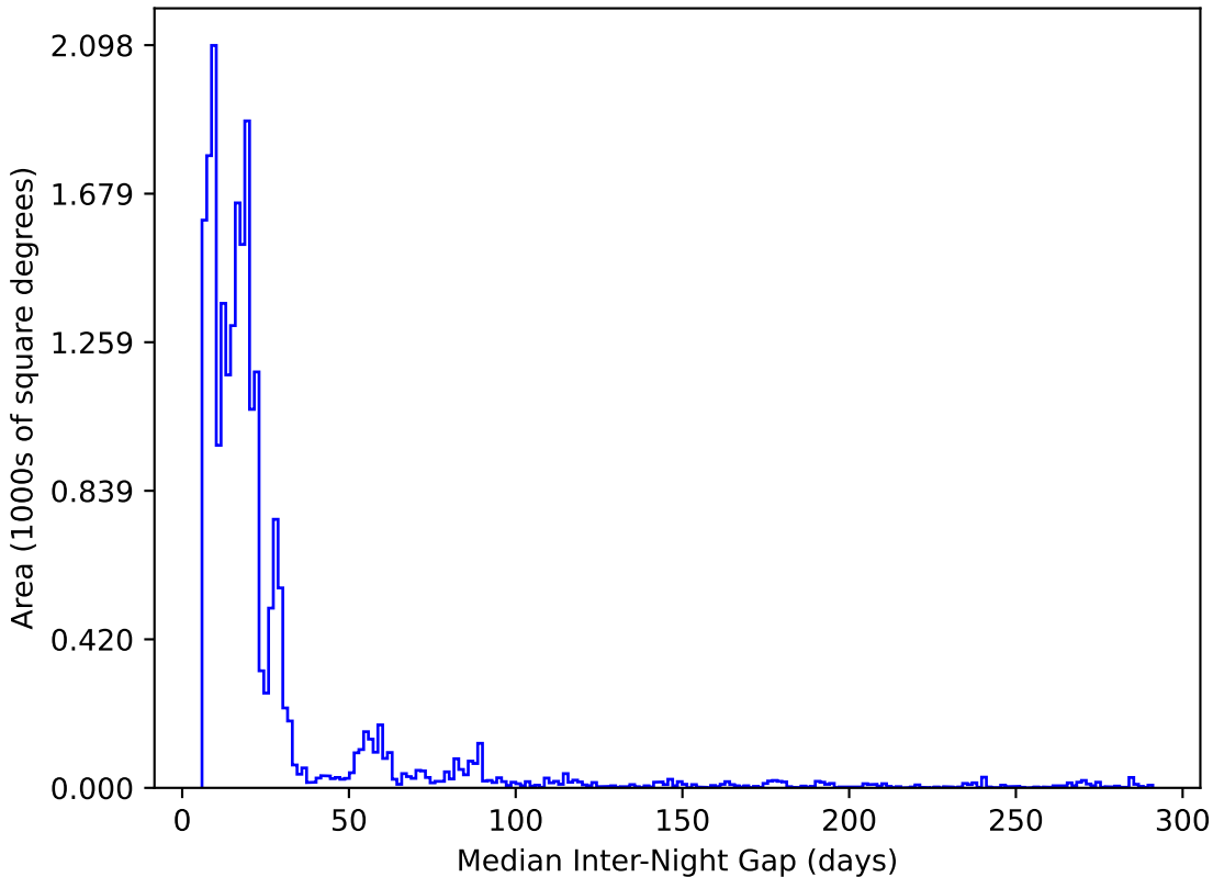
all_long_v3.4_10yrs All sky y band: Median Inter-Night Gap
