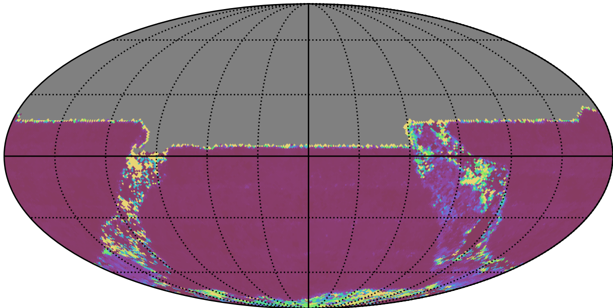
all_long_v3.4_10yrs All sky u band: Median Inter-Night Gap
