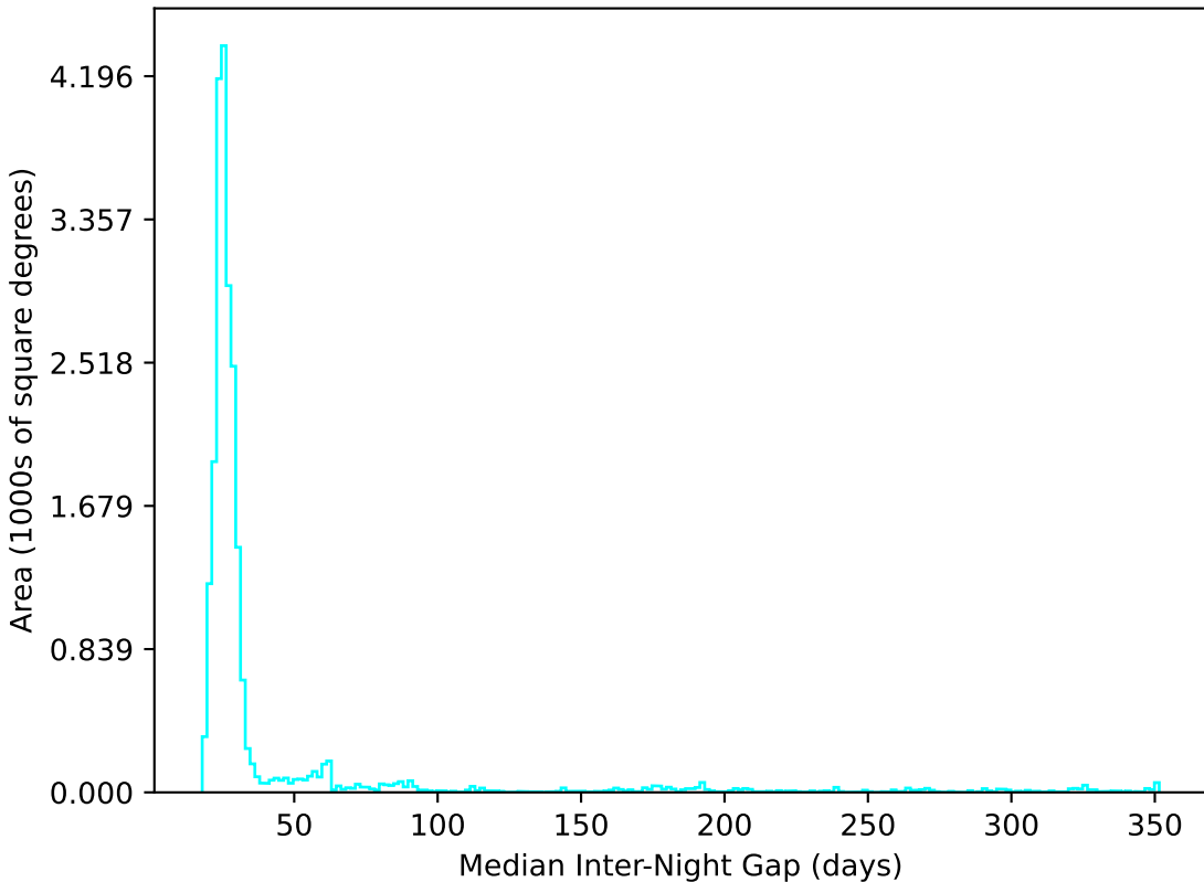
all_long_v3.4_10yrs All sky u band: Median Inter-Night Gap
