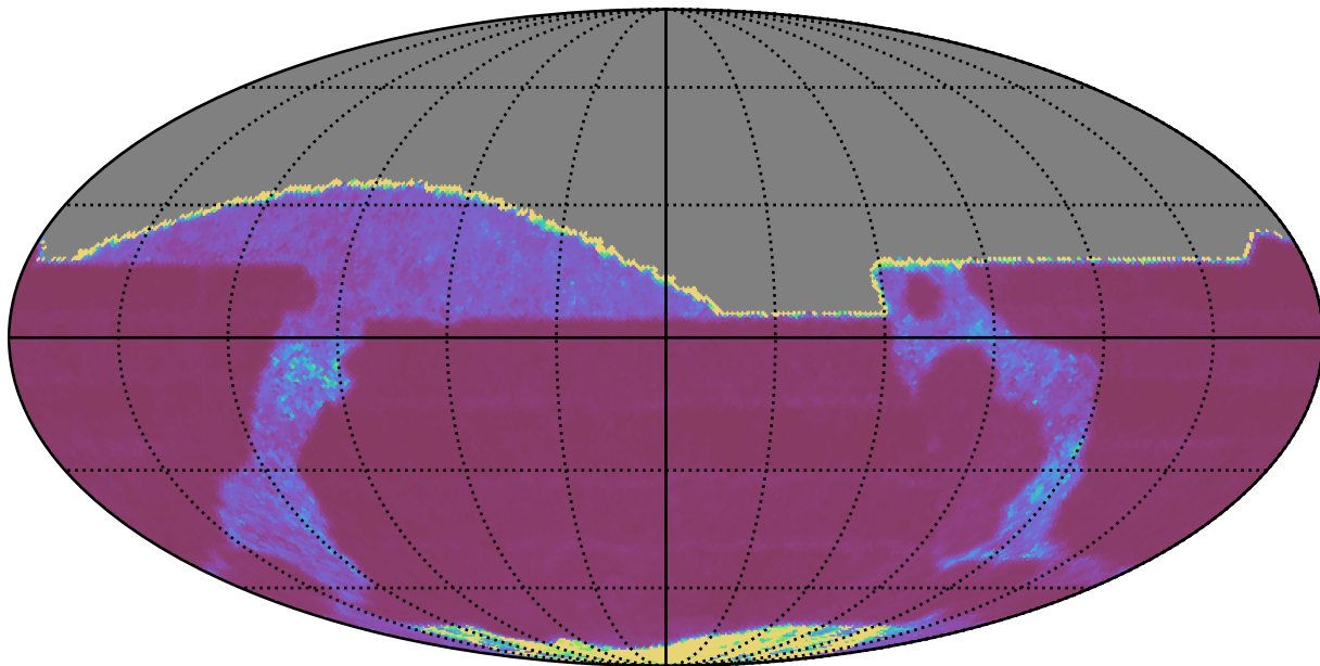
all_long_v3.4_10yrs All sky r band: Median Inter-Night Gap
