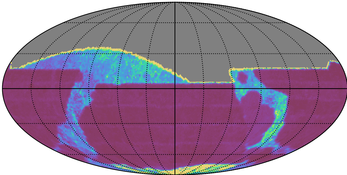
all_long_v3.4_10yrs All sky i band: Median Inter-Night Gap
