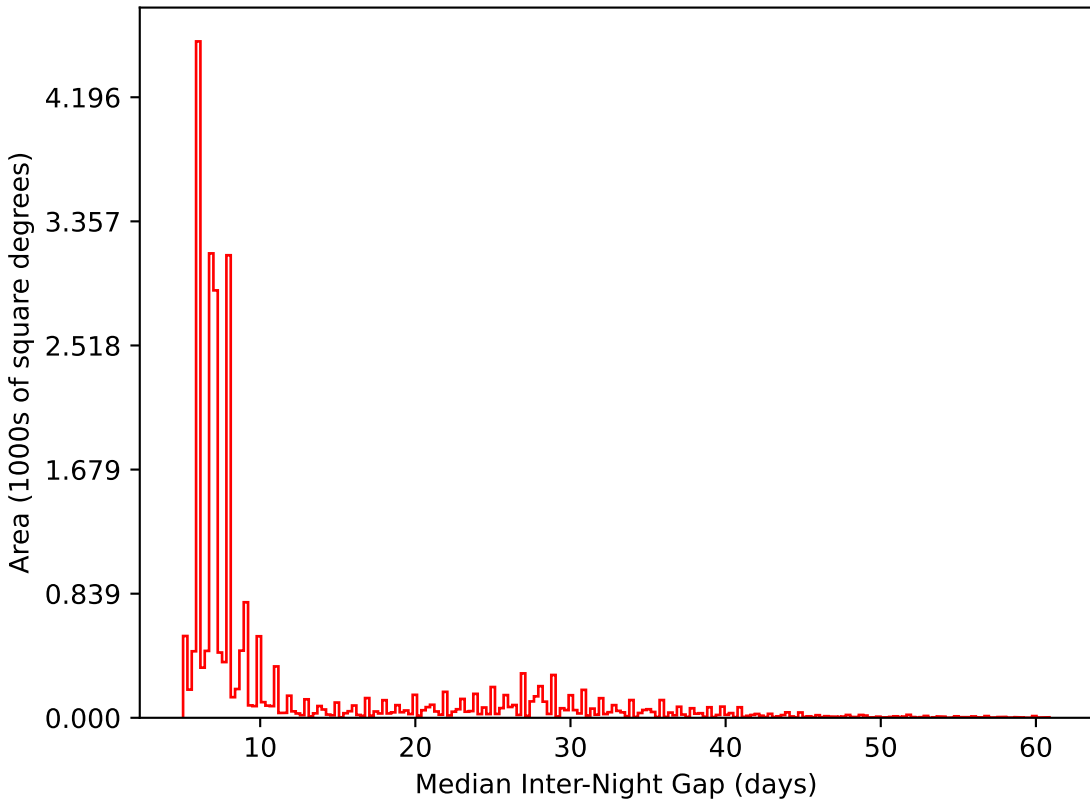
all_long_v3.4_10yrs All sky i band: Median Inter-Night Gap
