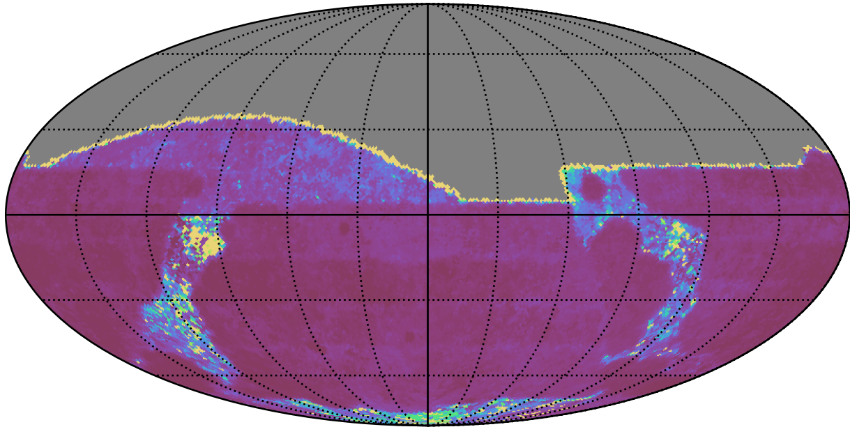
all_long_v3.4_10yrs All sky g band: Median Inter-Night Gap
