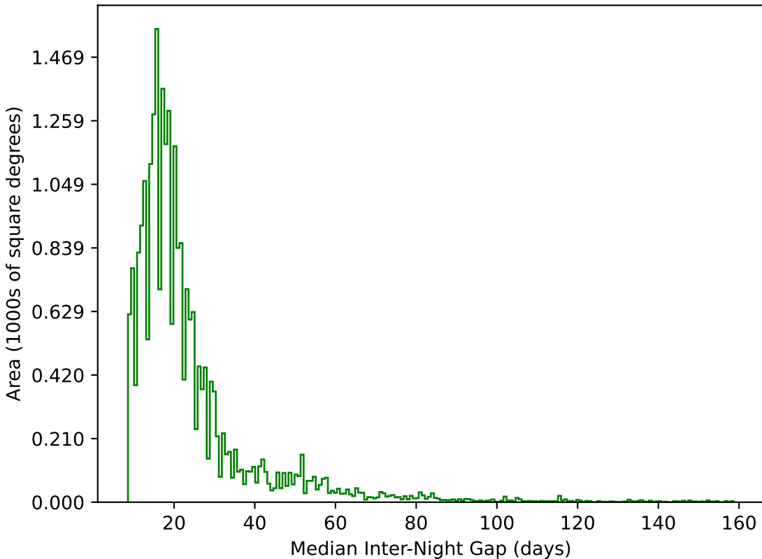
all_long_v3.4_10yrs All sky g band: Median Inter-Night Gap
