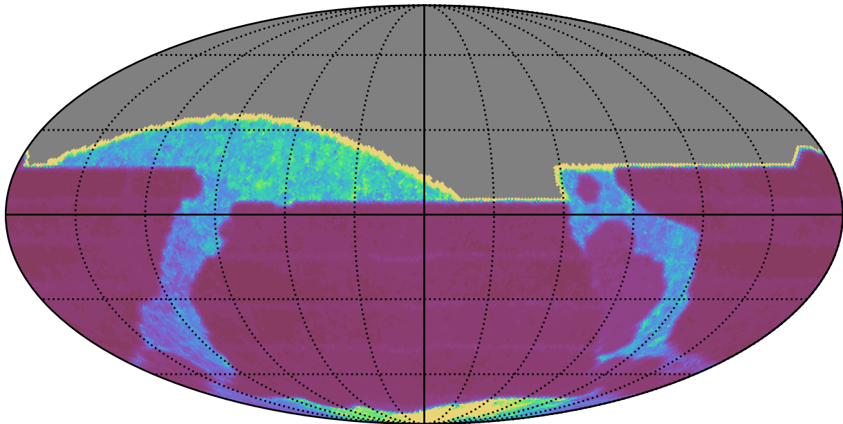
all_long_v3.4_10yrs All sky all bands: Median Inter-Night Gap
