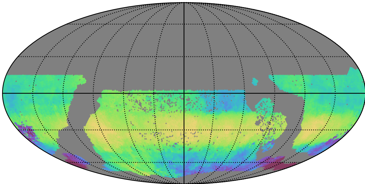
all_long_v3.4_10yrs WFD z band: Median HA
