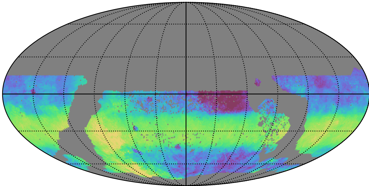
all_long_v3.4_10yrs WFD y band: Median HA
