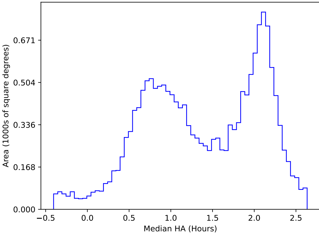
all_long_v3.4_10yrs WFD y band: Median HA
