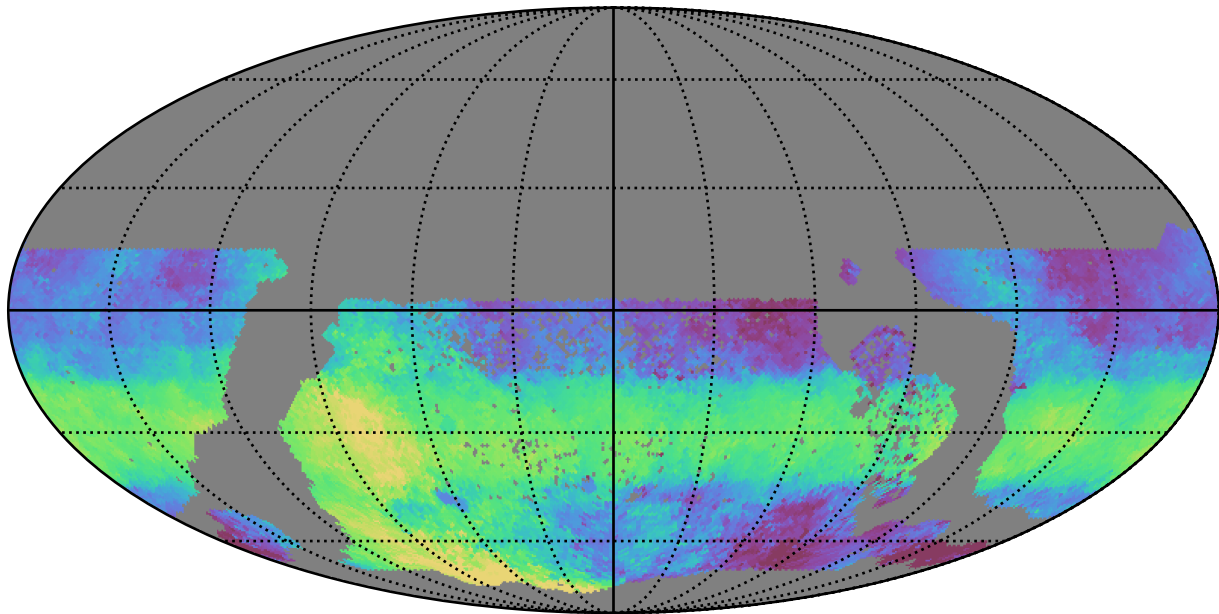
all_long_v3.4_10yrs WFD u band: Median HA
