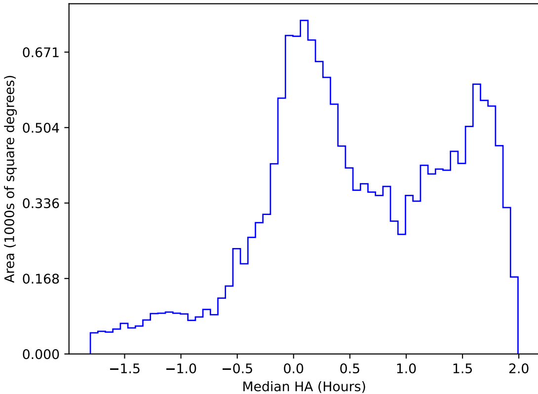
all_long_v3.4_10yrs WFD r band: Median HA
