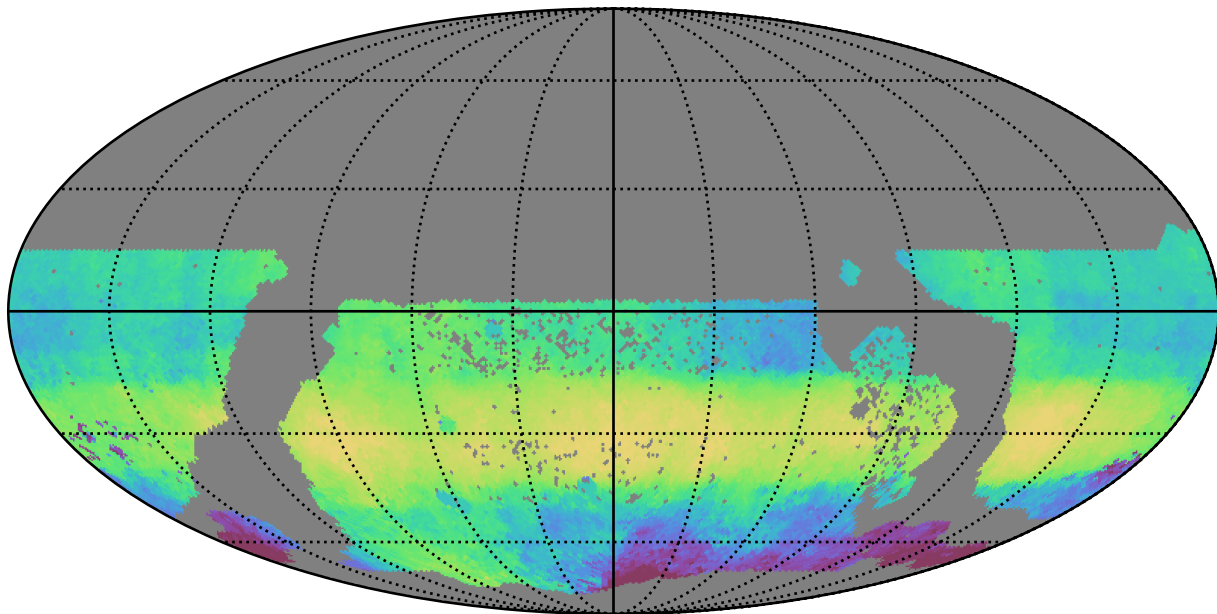
all_long_v3.4_10yrs WFD i band: Median HA
